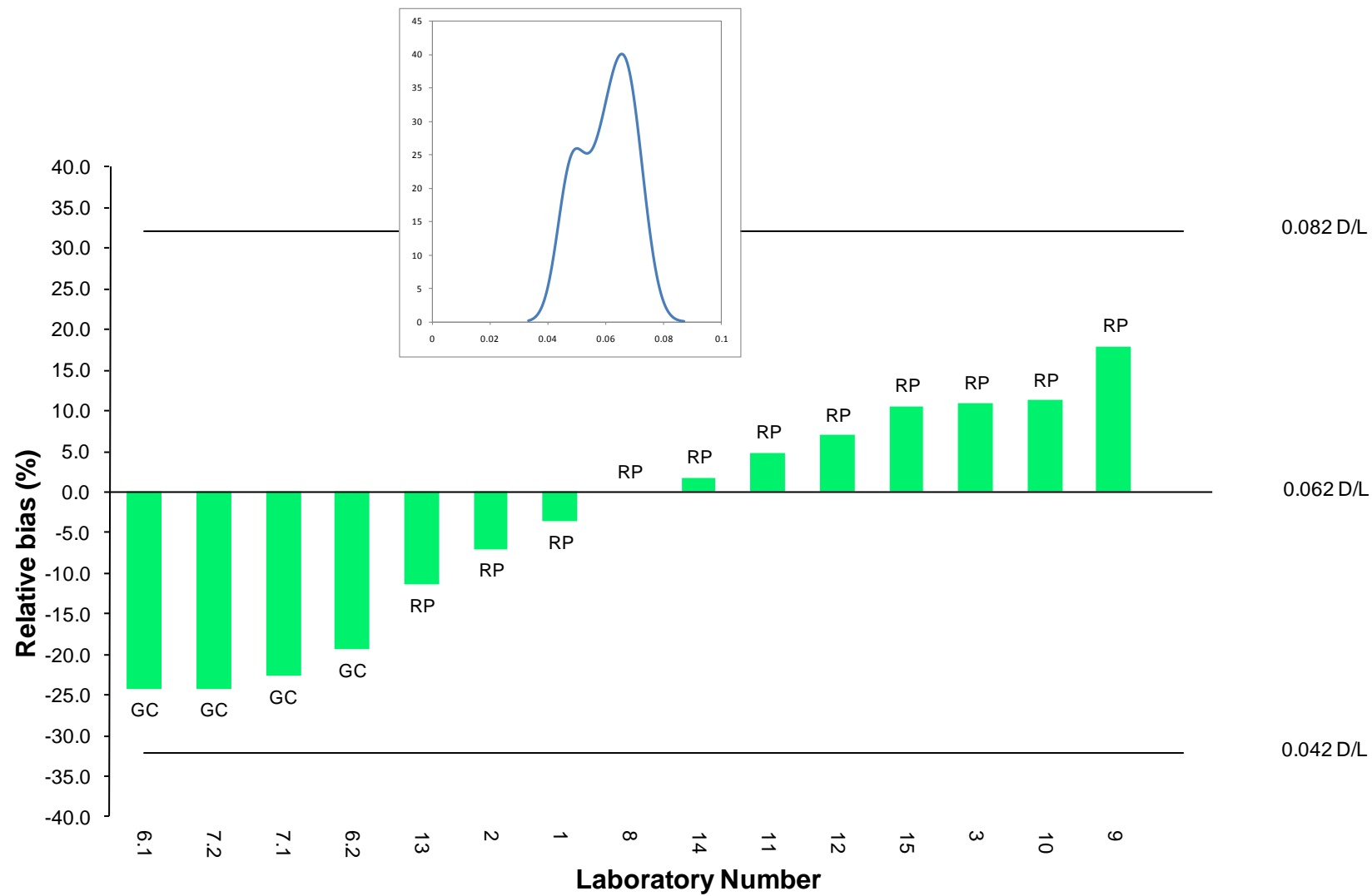
Figure 5.8: Relative Percentage Bias for Alanine D/L Results (all data) in Ostrich Egg Shell (B) Test Material
